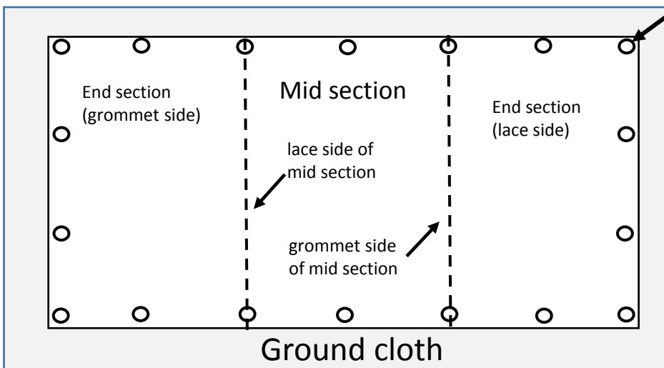
View from top of installation site
